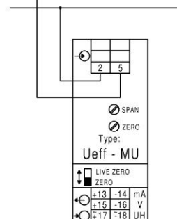
Spannungsmessung (TrueRMS) voltage measuring (TrueRMS)
