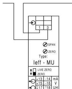
Strommessung (TrueRMS) current measuring (TrueRMS)
